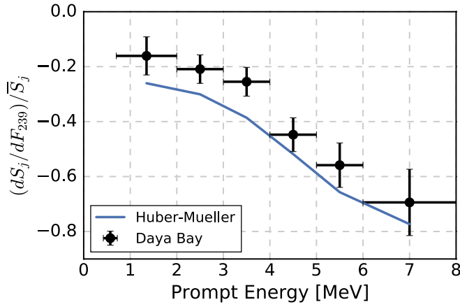
FIG. 5. Fractional variations in IBD yield (1/\bar{\sigma}_j)(dS_j/dF_{239}) for different prompt energy E_p ranges for Daya Bay data and for the Huber-Mueller model. The variation of the slope (1/\bar{\sigma}_j)(dS_j/dF_{239}) with energy, which indicates evolution-dependent changes in the antineutrino spectrum, appears consistent between the data and predictions.
