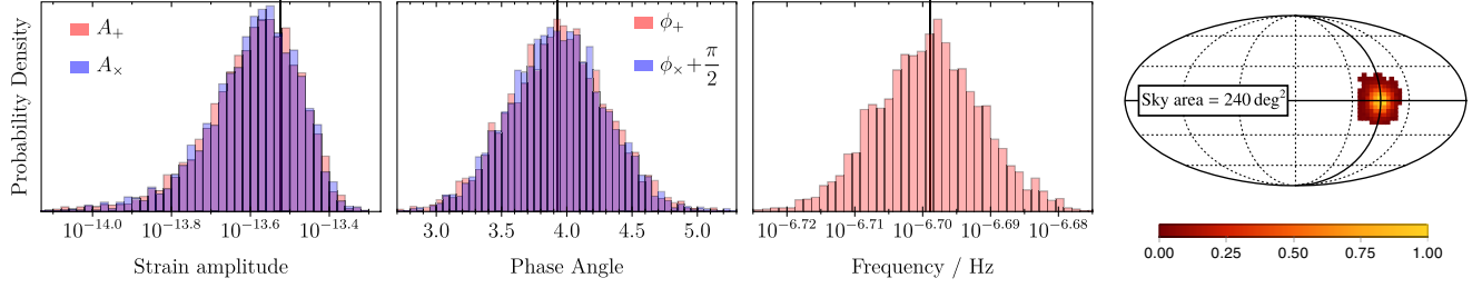
FIG. 2. One-dimensional marginalized posteriors on \tilde{\Psi} (black lines indicate injected values). The injected GW was circularly polarized (i.e., \phi_+ - \phi_\times = \pi/2 ) so the \phi_\times posterior is shifted such that it overlaps with \phi_+ . The Mollweide sky map is shown with the area of the 68% credible region given.
